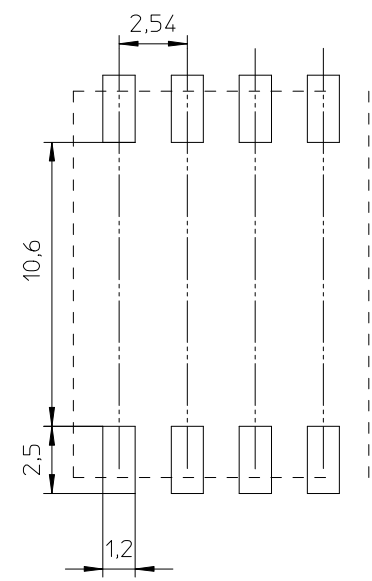
PROPOSED PAD ARRANGEMENT:
