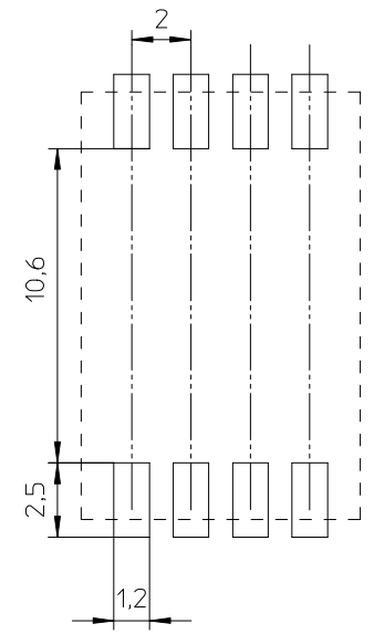
PROPOSED PAD ARRANGEMENT:
