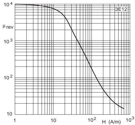
Fig.4 Reversible permeability as a function of magnetic field strength.
