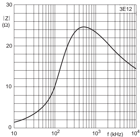
Fig. 6 Impedance as a function of frequency measured on toroid T25/15/10.
