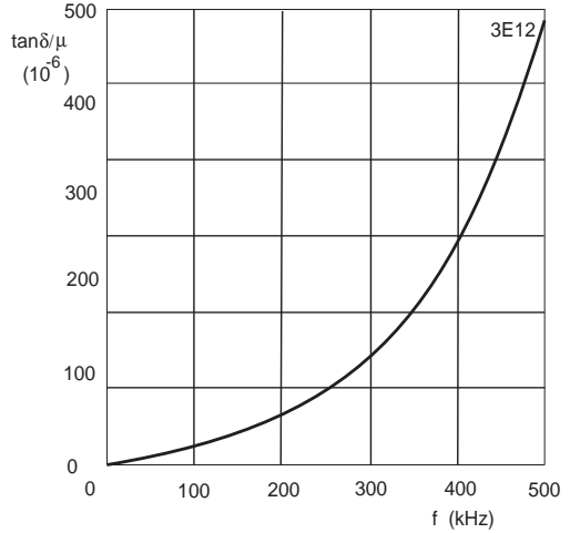
Fig.5 Loss factor as a function of frequency.
